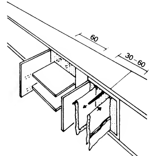
⑭ Equipment cupboard and towel cupboard
